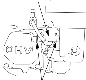
TUBE CLIP
